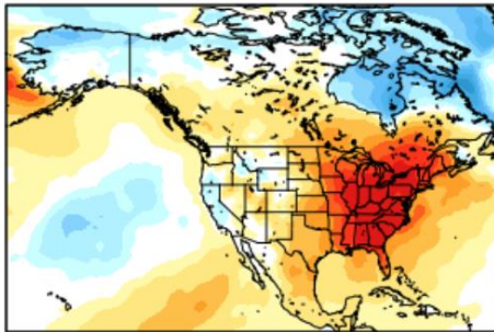
MME (63 Ensemble Members)
