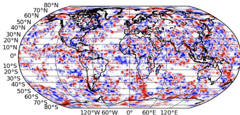
Shallow Convection
