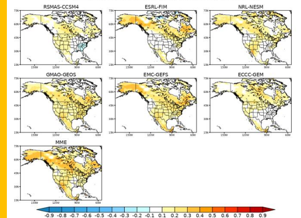
SubX Week 3 Anomaly Correlation 2m Temperature [ SON 1999-2014 ]
